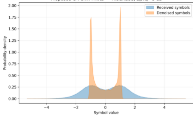
(c) Rician LOS
