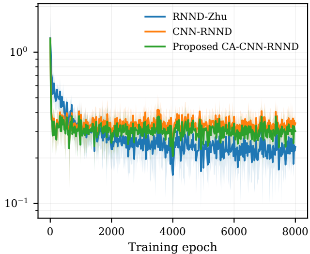
Denoising MSE
