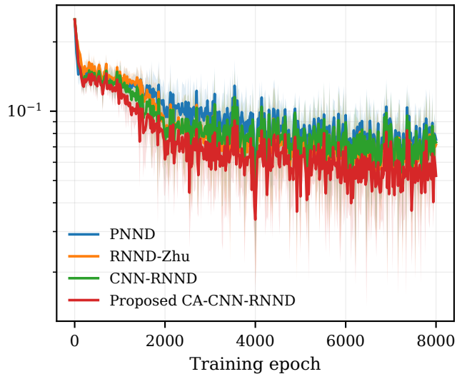
Decoding loss
