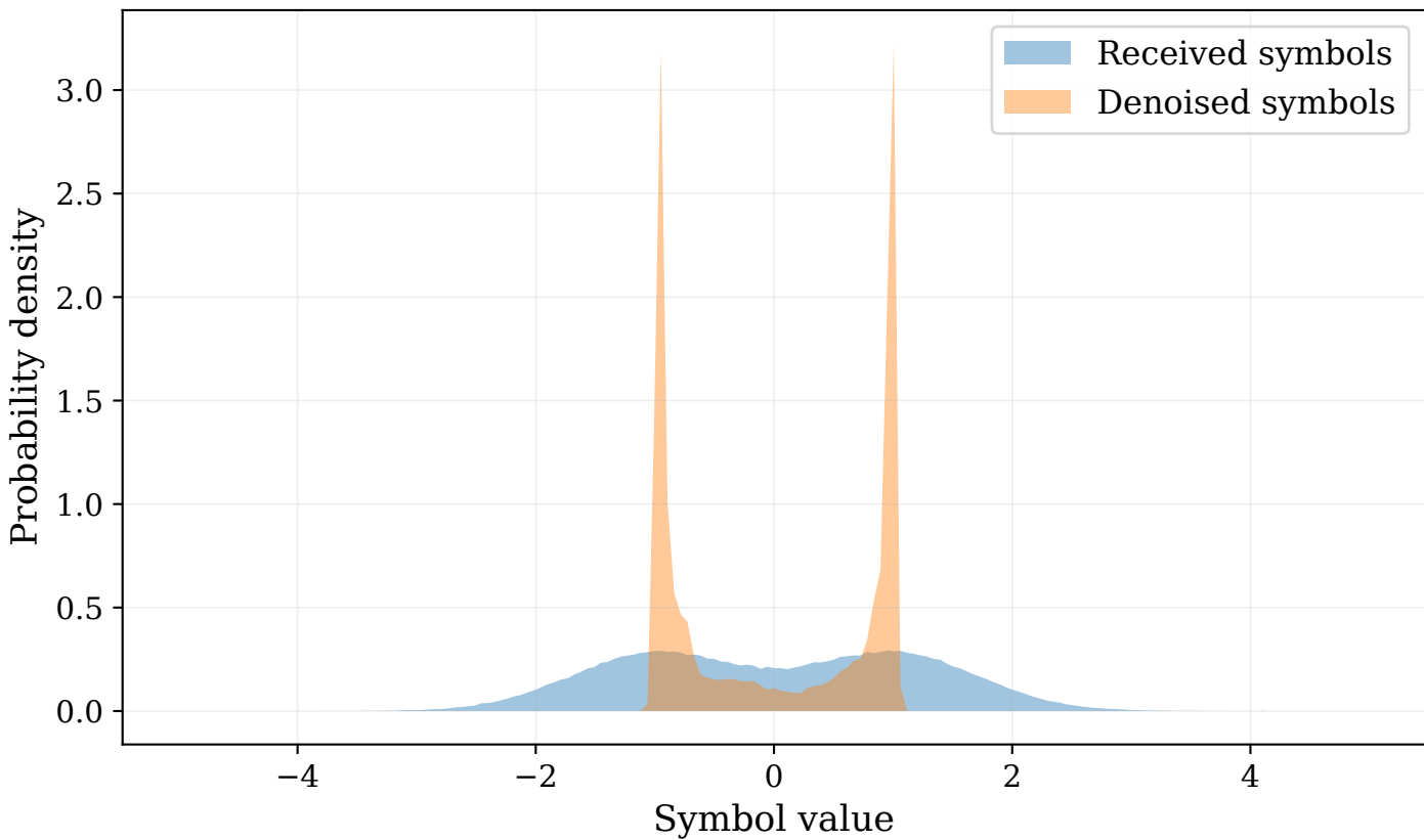
Proposed — AWGN, E_b/N_0 = 3 dB
