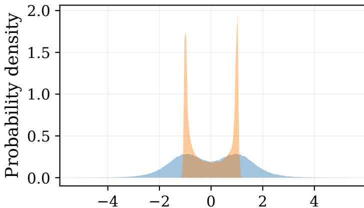
(c) Rician LOS
