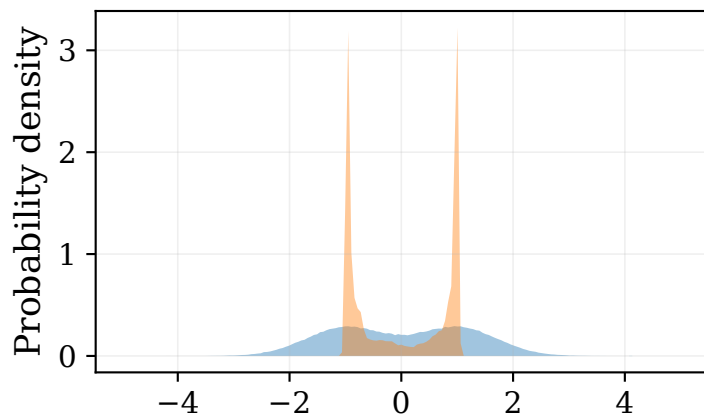
(a) AWGN
