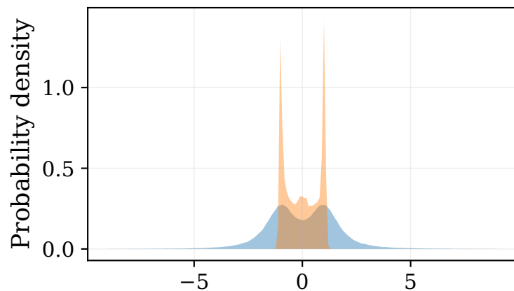
(b) Rayleigh
