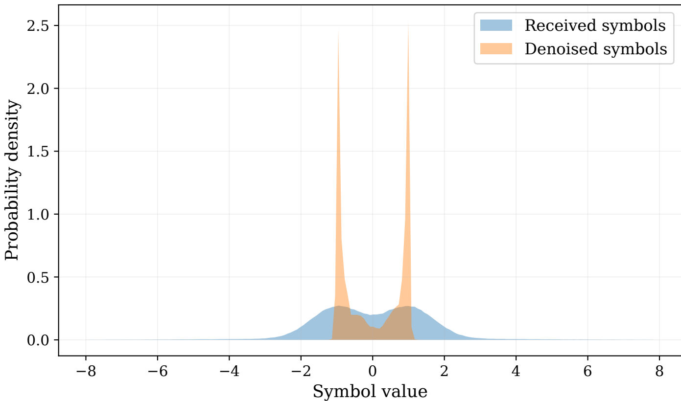
Proposed — Impulsive, E_b/N_0 = 3 dB
