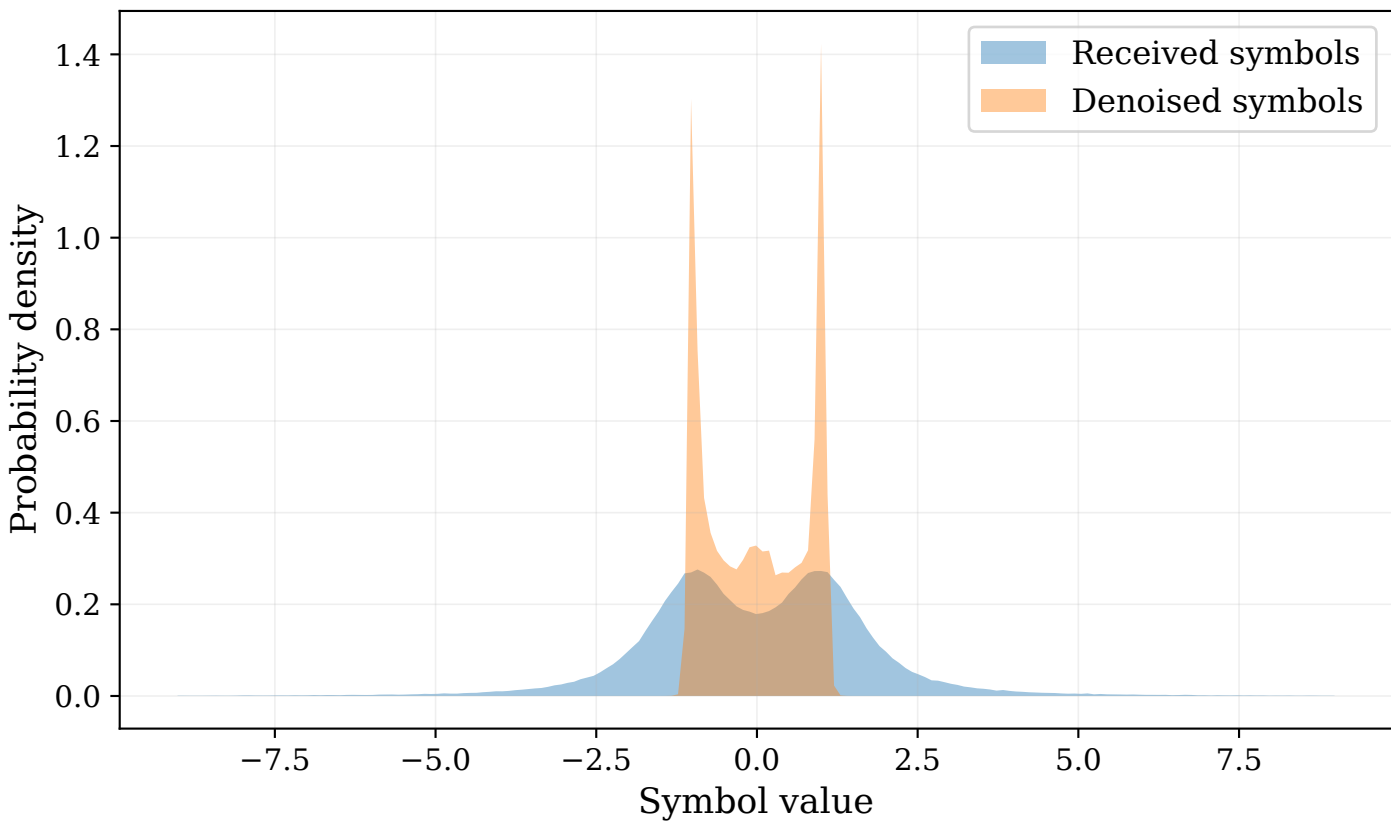
Proposed — Rayleigh, E_b/N_0 = 3 dB
