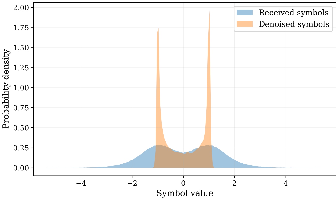
Proposed — Rician LOS, E_b/N_0 = 3 dB
