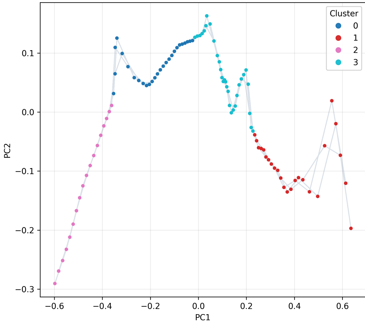
Flow Latent Trajectory + KMeans Segmentation
