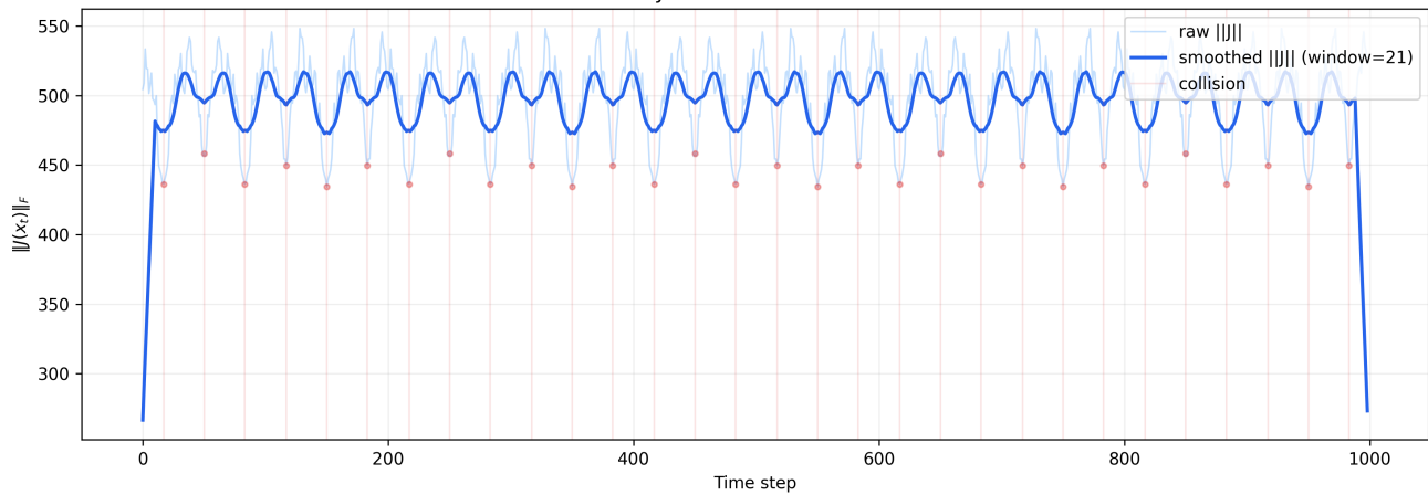
Flow Jacobian norm over time
