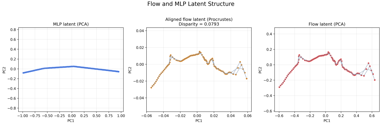
Figure 6. Flow-model comparison, showing that the segmentation survives an invertible reparameterization (flow samples Procrustes-aligned to model/latent.npy ; N=999 ; Procrustes with scaling).
