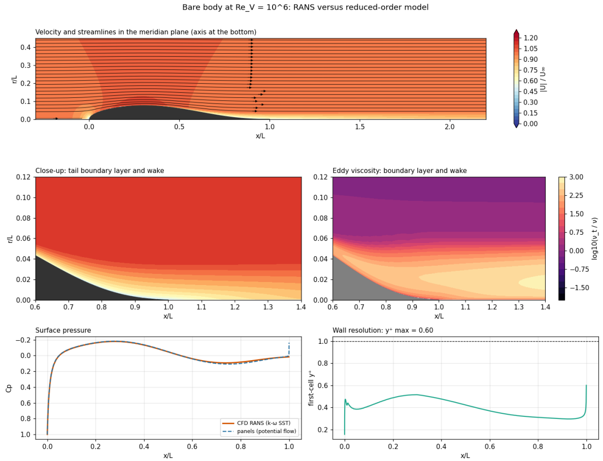
Figure 5: RANS versus reduced-order model, bare body at Re_V = 10^6 .
