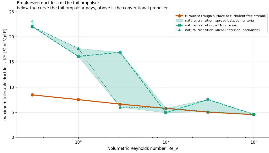
Figure 4: Break-even duct loss K^* versus Re_V . Solid line: fully turbulent boundary layer (result). Shaded band: spread between transition criteria for natural transition, shown for information only (not a result).
