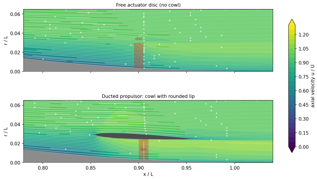
Figure 6: Flow near the tail with the ducted intake (case D).
