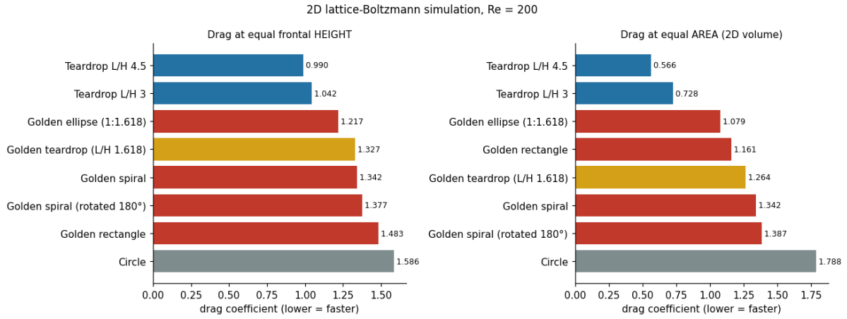
Figure 1: 2D lattice-Boltzmann drag at Re = 200 for golden-ratio shapes and teardrops.
