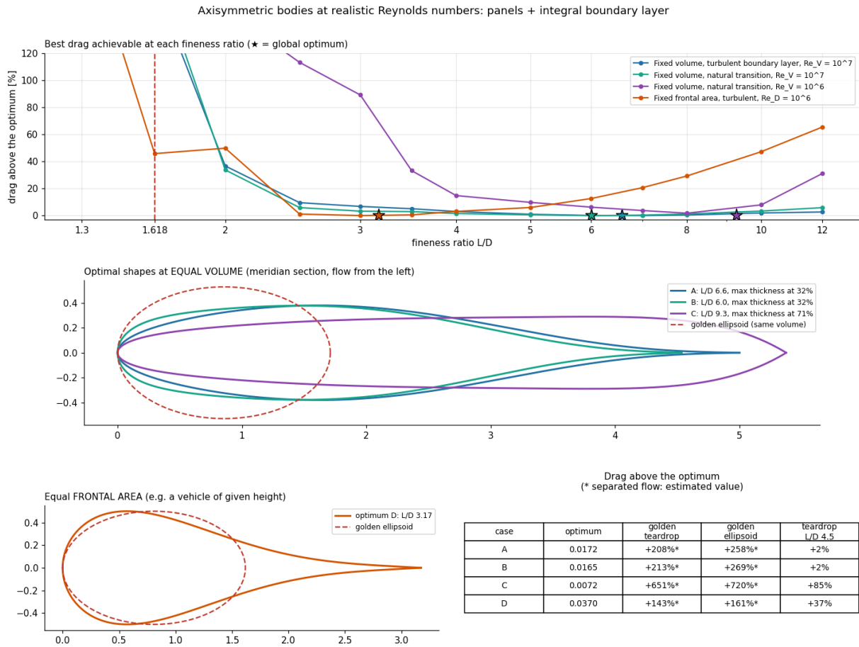
Figure 2: Axisymmetric optimal bodies.
