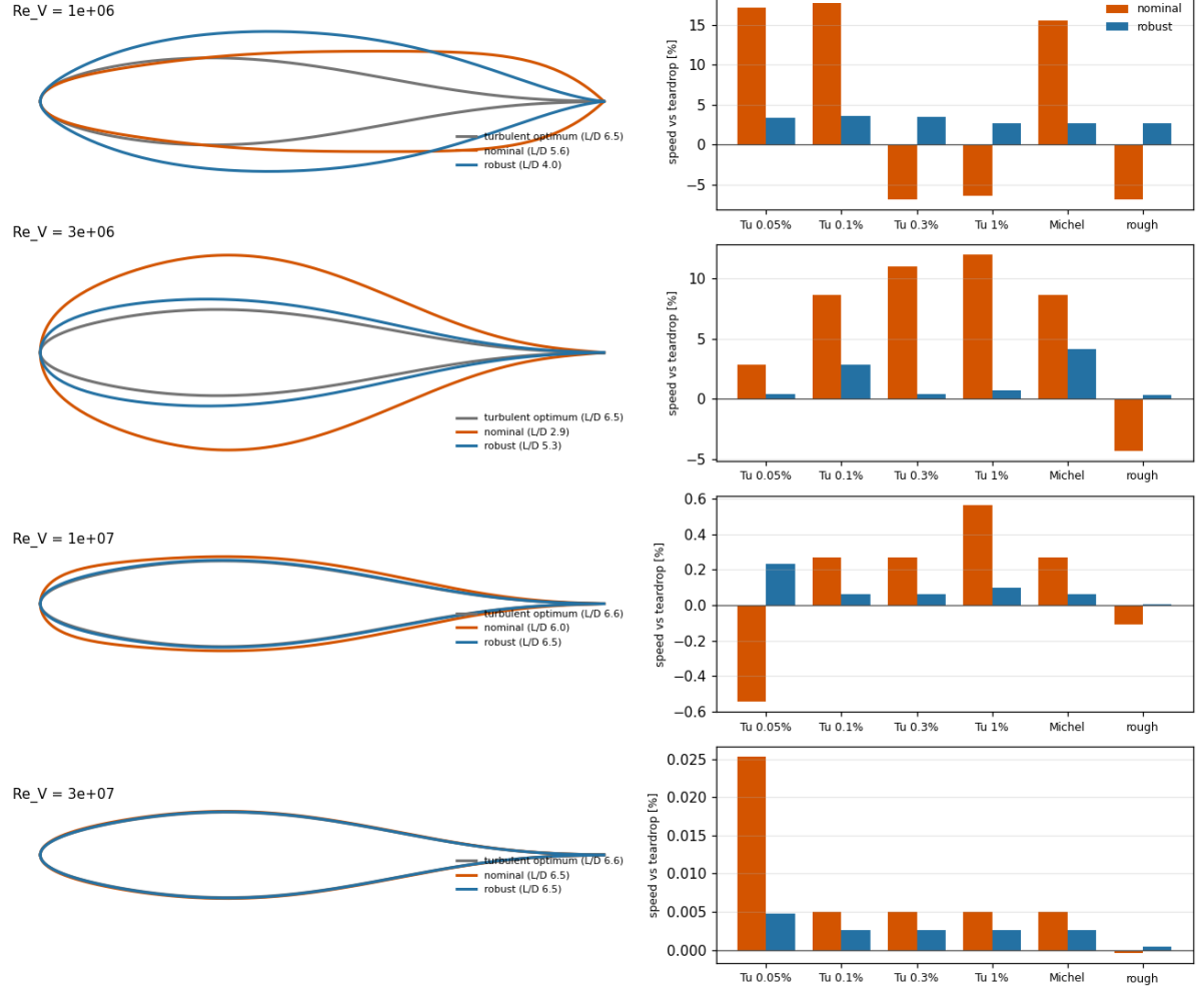
Optimal shape with natural transition: nominal vs guaranteed (same power)
