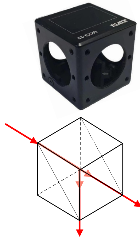
(c) Spatial-domain alignment device
