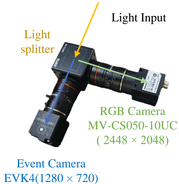
(a) The setup of our dataset collection
