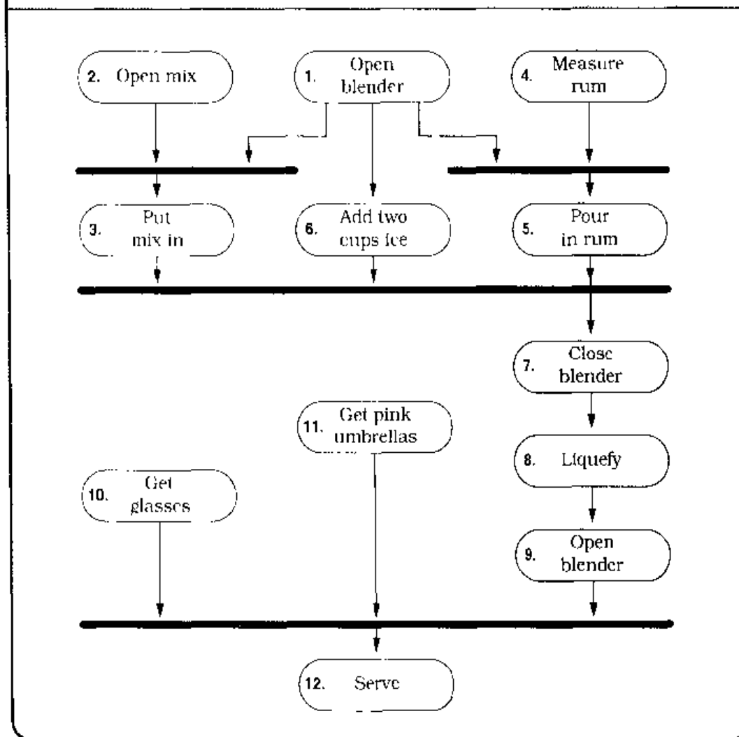
Figure 5.2. UML activity diagram: making a piña colada
