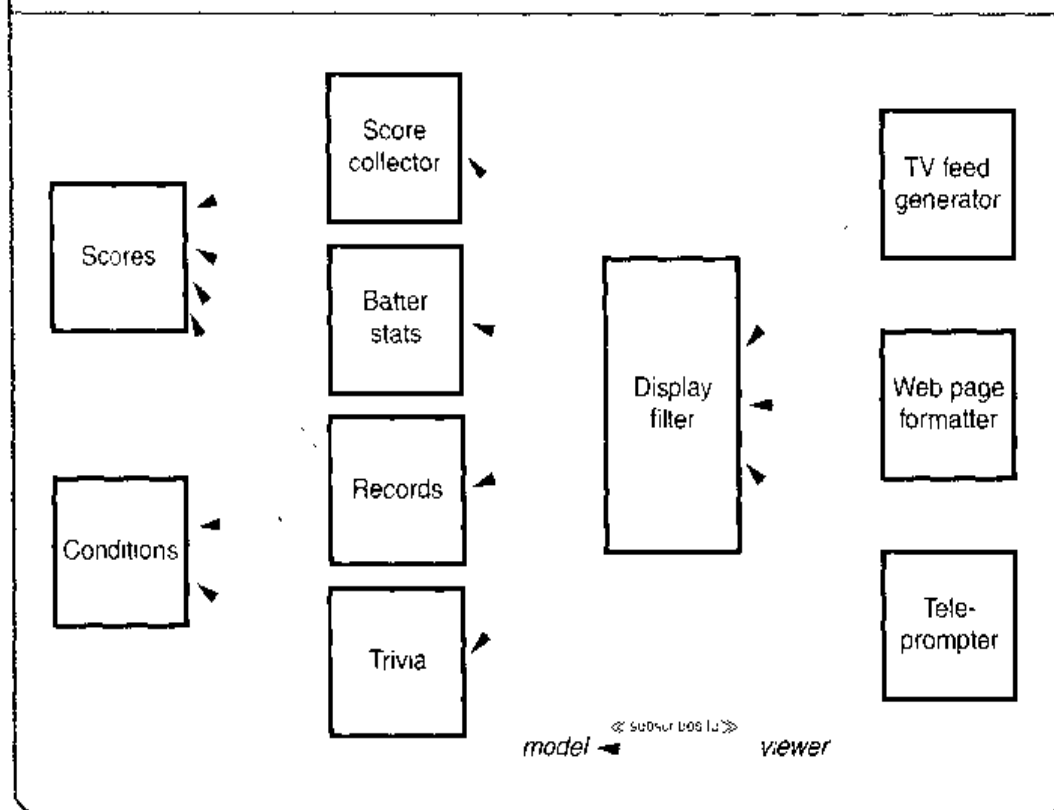
Figure 5.5. Baseball reporting. Viewers subscribe to models.
