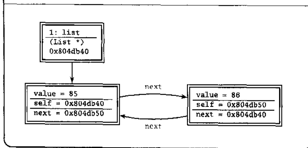
Figure 3.2. Sample debugger diagram of a circular linked list. The arrows represent pointers to nodes.
