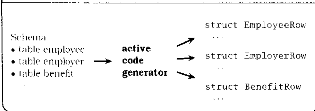
Figure 3.3. Active code generator creates code from a database schema
