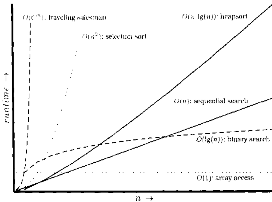
Figure 6.1. Runtimes of various algorithms
