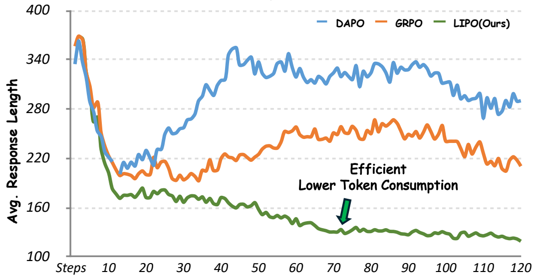
(b) Evolution of mean response length across methods during training process
