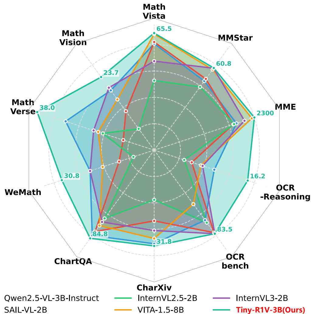
(c) Comparison with other reasoning MLLMs.
