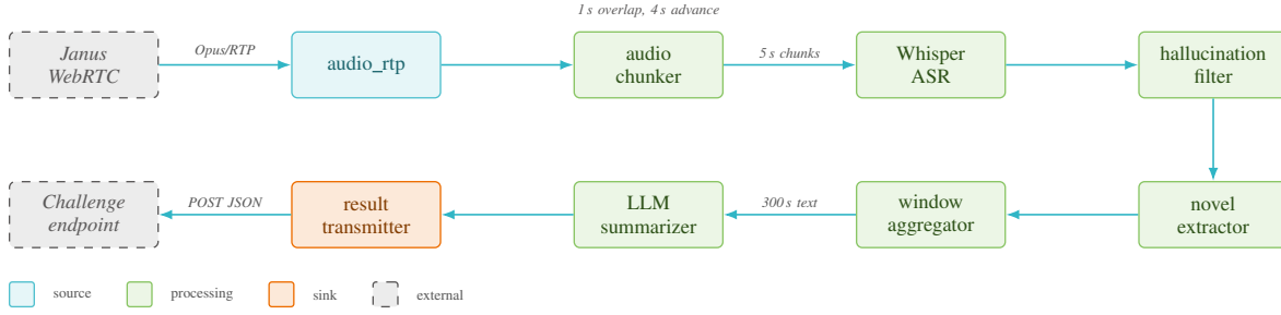
Fig. 1: End-to-end STREAMIND pipeline. Janus delivers mono Opus/RTP into audio_rtp ; chunks slide every 4s through ASR; deduplication and hallucination filtering precede a 300s aggregation buffer; the summarizer emits {summary, keywords[3]} per window; the sink stores locally and POSTs to the challenge endpoint.
