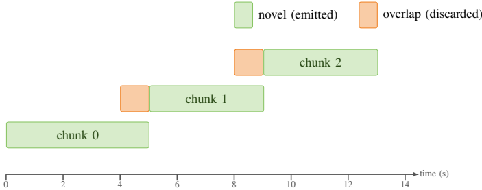
Fig. 3: Audio chunking and novel extraction timing. Five-second chunks slide by 4s; the novel extractor isolates the 4s of newly-spoken content each step, dropping the 1s of overlap with the previous chunk.
