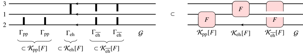
FIG. 2. Regrouping of the iterated Eq. (17) into the Faddeev series. Left: one term of the iteration, a sequence of pair vertices \mathcal{K}_\alpha[\Gamma_\alpha] (thick bars). Right: each sequence of consecutive vertices in the same pair is part of the full two-body scattering \mathcal{K}_\alpha[F] of that pair (shaded box), so that consecutive boxes always belong to different pairs.
