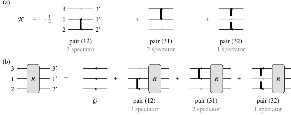
FIG. 1. (a) The Faddeev kernel, Eqs. (15) and (16). Lines run from the second triple on the right to the first triple on the left. The thick bar is the two-particle vertex \Gamma^{\text{pp}} : it connects the two lines of one pair, while the third line (gray) is a spectator that passes the vertex without interacting. (b) The Dyson equation for R , Eq. (15), sorted by the interacting pair. The exchange of the lines 1 and 2 in \mathcal{G} is implied.
