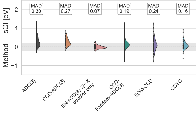
FIG. 4. Errors of the IPs with respect to sCI (aug-cc-pVQZ) for ADC(3), CCD-ADC(3), EN-ADC(3), CCD-Faddeev-ADC(3) and CCSD, over the 48 states of the first block of Table IV.
