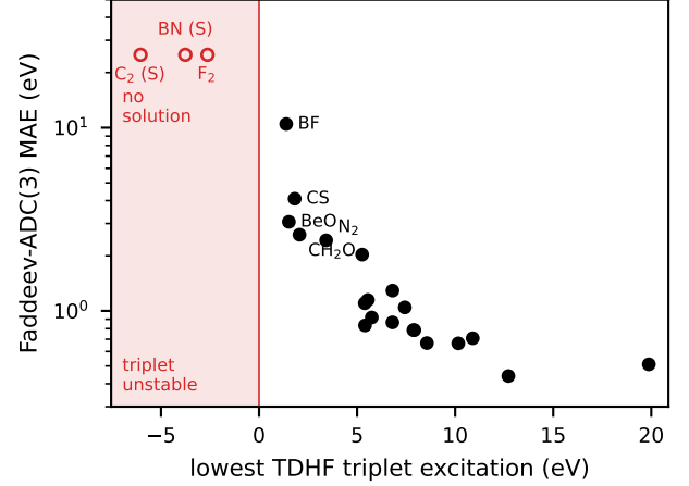
FIG. 5. Mean absolute error per molecule of Faddeev-ADC(3) (RPA pair channels) against sCI, versus the lowest TDHF triplet excitation energy of the RHF reference (aug-cc-pVDZ). For unstable references, where Faddeev-ADC(3) has no solution (open circles), the most negative eigenvalue of A \pm B is shown; (S): also unstable in the singlet channel.
