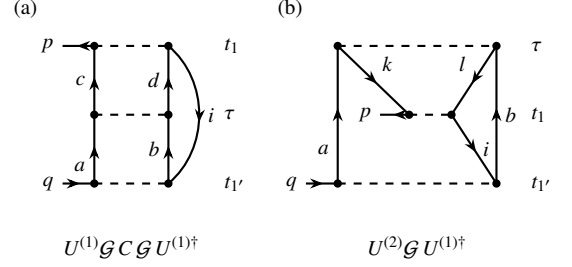
FIG. 3. Time-ordered third-order self-energy diagrams with one pp rung (block II, time upward, dashed lines: bare interactions, external legs drawn horizontally, so that each horizontal cut between two interactions crosses only the lines of one intermediate state). (a) Rung at t_{1'} < \tau < t_1 : the pair propagates in \mathcal{P} . (b) Rung at \tau > t_1 : at t_1 , the pair slot holds the holes k and l , the reversed configuration (kl; i) in \bar{\mathcal{P}}_{\text{pp}} , and the rung gives the first-order amplitude t_{kl}^{ab} of U^{(2)} .
