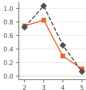
SiH 4 , IP 1 (sCI 12.68 eV)
