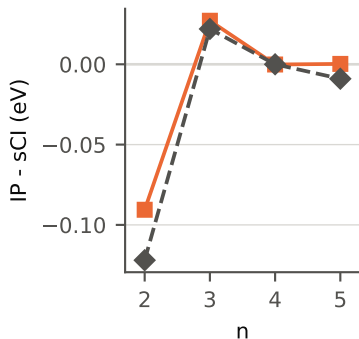
PH 3 , IP 2 (sCI 13.62 eV)
