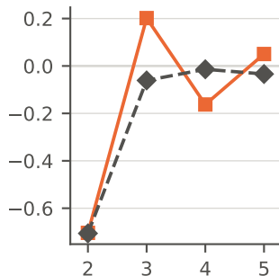
PH 3 , IP 3 (sCI 19.45 eV)
