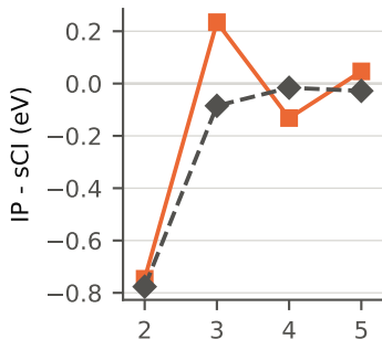
PH 3 , IP 2 (sCI 13.62 eV)
