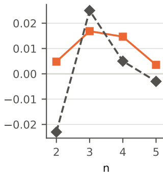
SiH 4 , IP 1 (sCI 12.68 eV)
