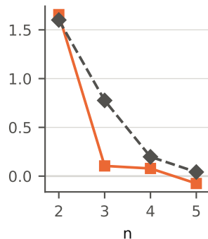
PH 3 , IP 3 (sCI 19.45 eV)
