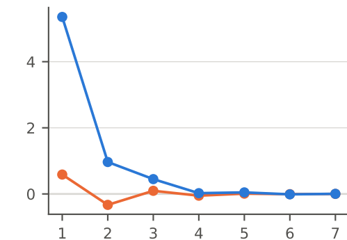
Ar, aug-cc-pVDZ, 1s2s2p frozen
