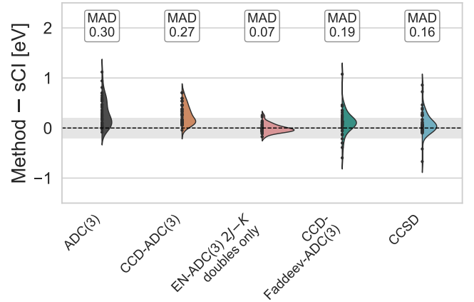
FIG. 4. Errors of the IPs with respect to sCI (aug-cc-pVQZ) for ADC(3), CCD-ADC(3), EN-ADC(3), CCD-Faddeev-ADC(3) and CCSD, over the 48 states of the first block of Table IV.
