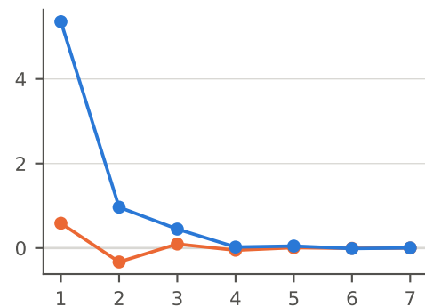
Ar, aug-cc-pVDZ, 1s2s2p frozen
