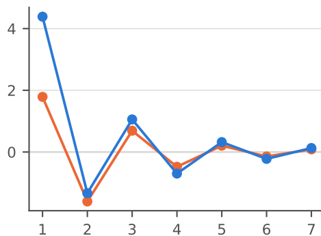
Ne, aug-cc-pVDZ, 1s frozen
