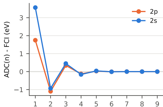
Ne, cc-pVDZ, 1s frozen
