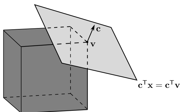
Figure 2.3: A supporting hyperplane exposing a vertex of a polyhedron.
