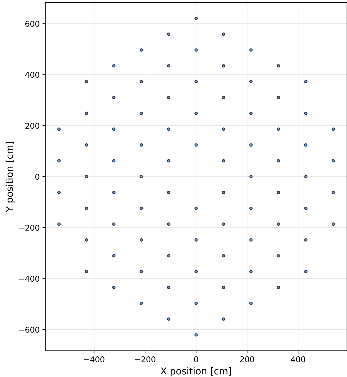
Mirror positions - MST
