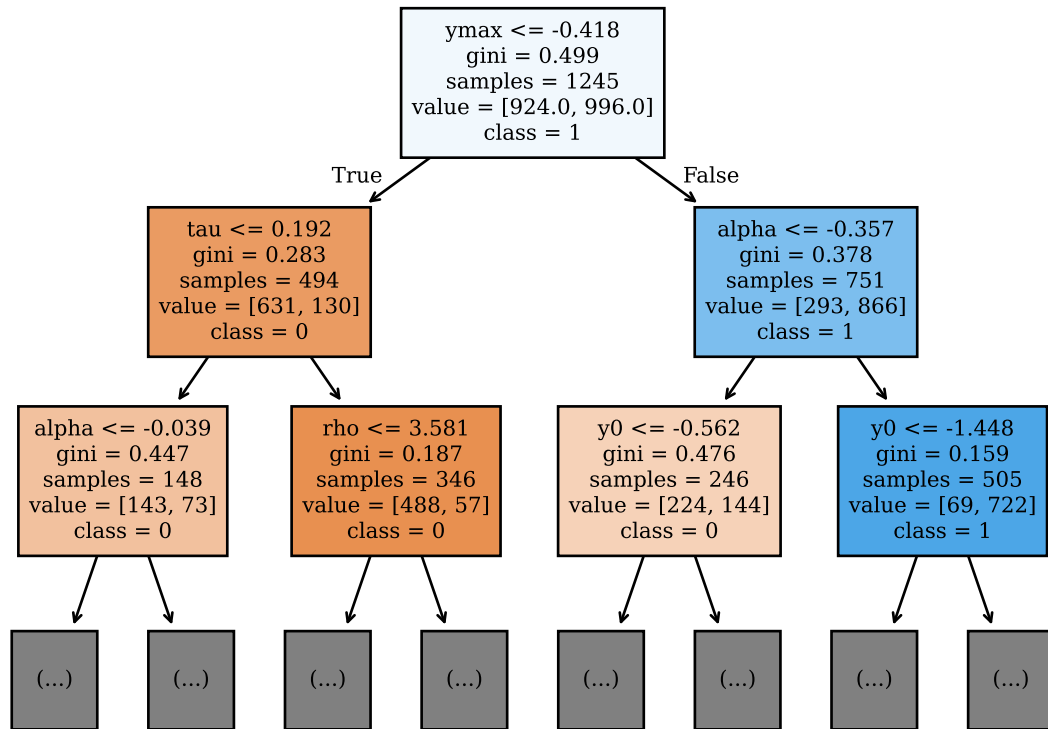
Best Tree for HP F1 Score: 0.83, Depth: 18, Leaves: 198
