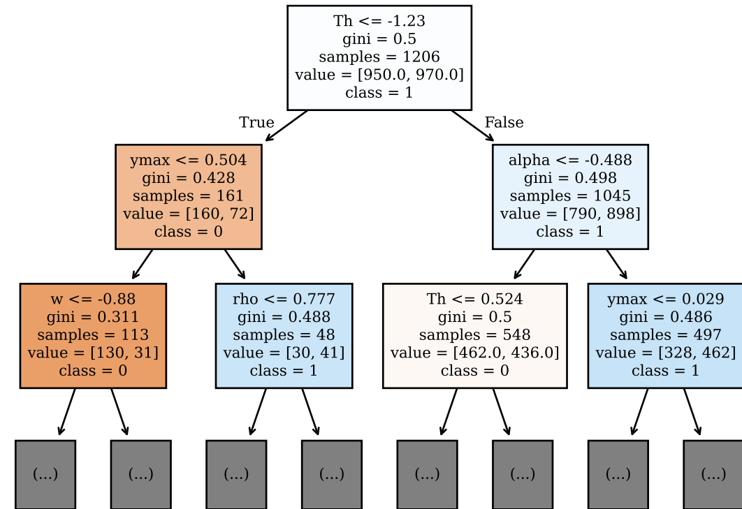
Best Tree for EV F1 Score: 0.71, Depth: 18, Leaves: 276
