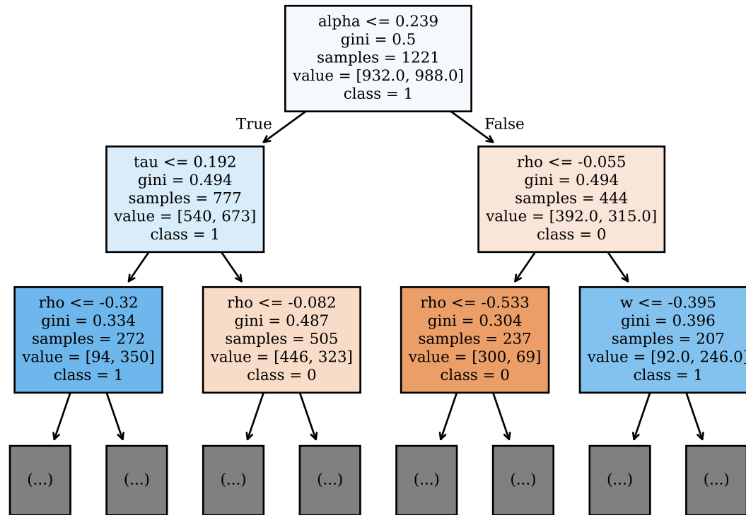
Best Tree for PV F1 Score: 0.80, Depth: 14, Leaves: 210
