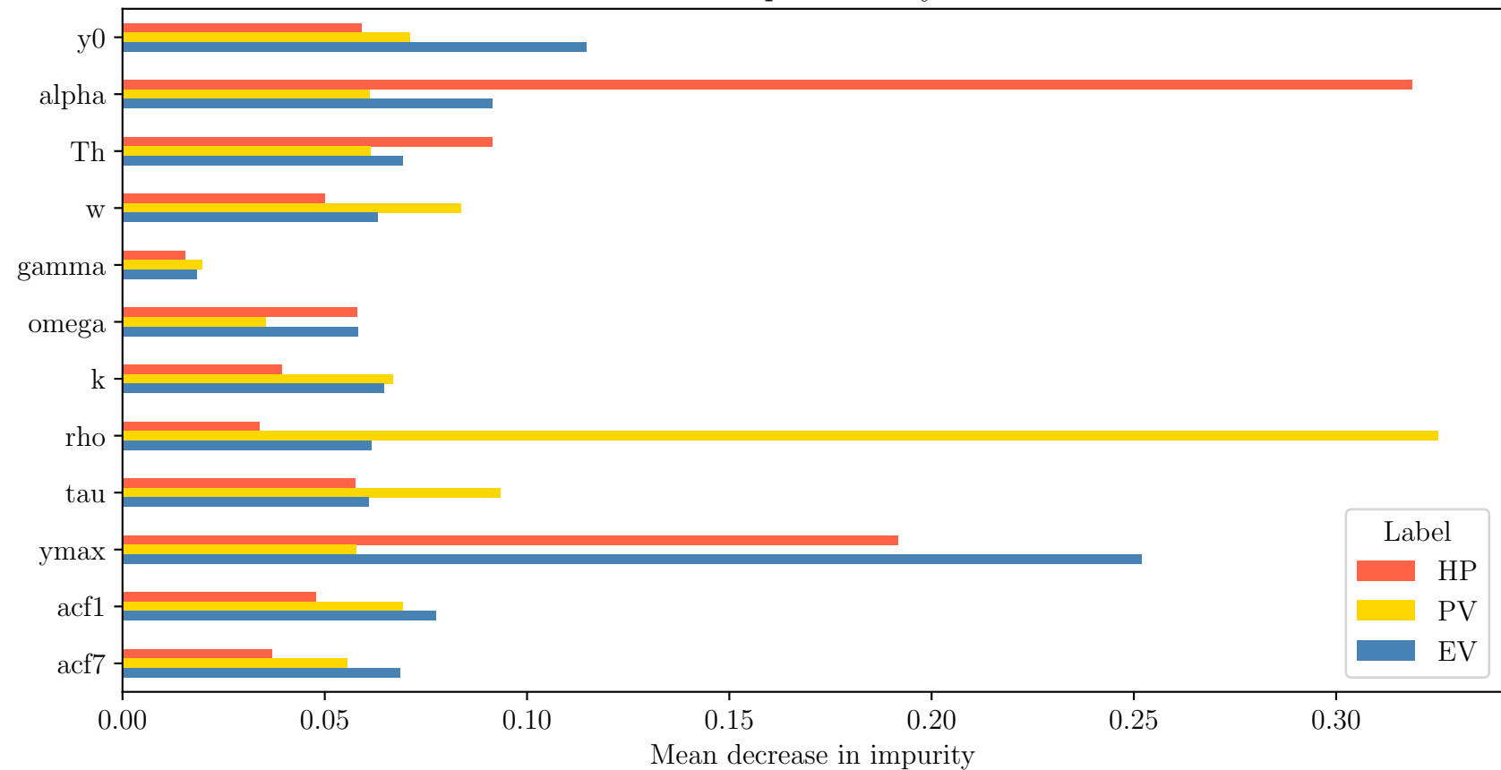
Feature importance by label
