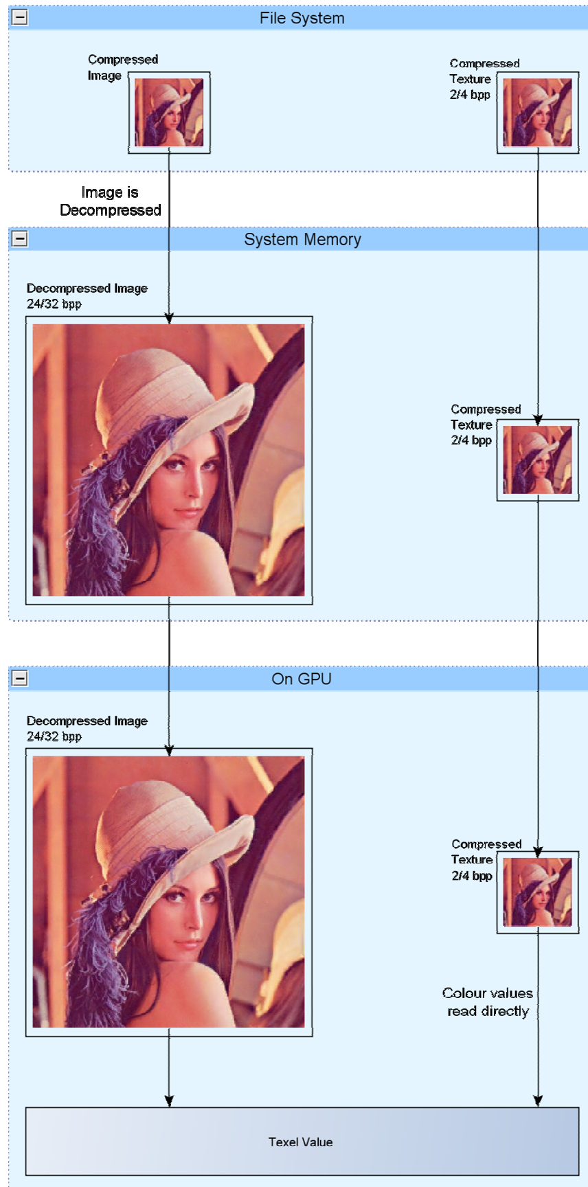
Figure 5-1 Image File Compression vs. Texture Compression
