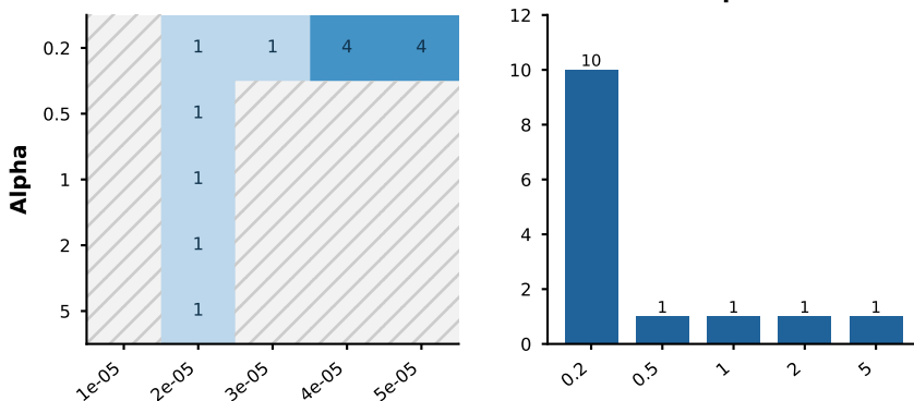
Alpha
