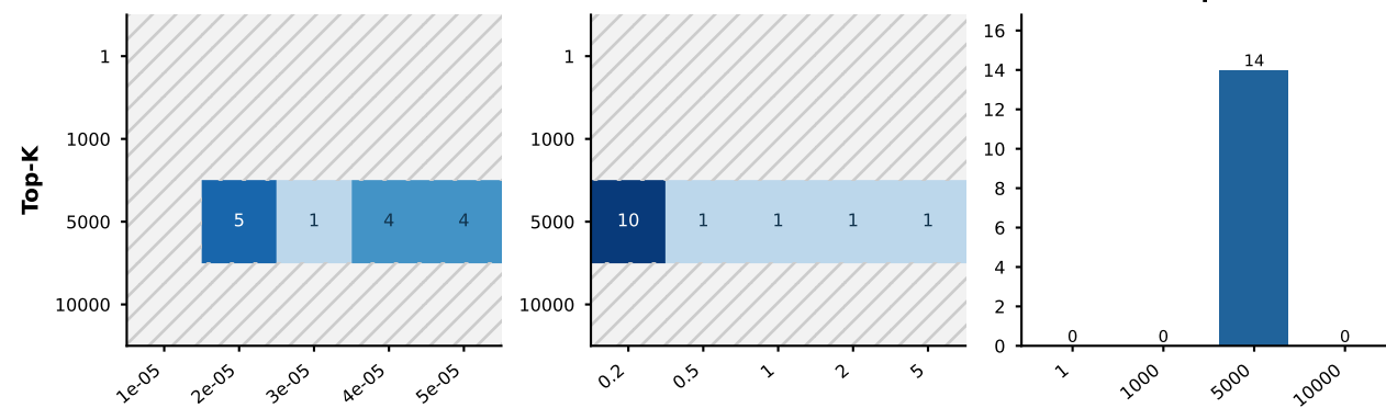
Top-K
