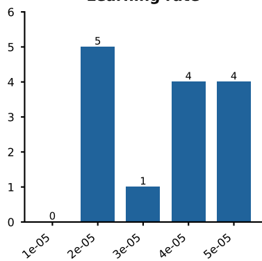
Learning rate
