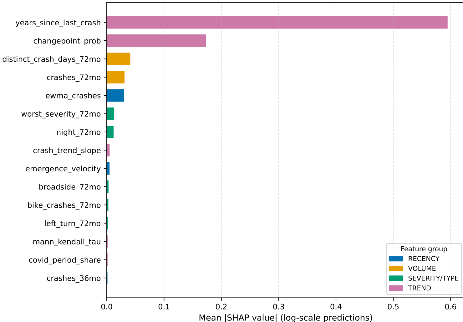
Top-15 Feature Importance — Crash-Only XGBoost Tweedie (locked M3a model, random test split)
