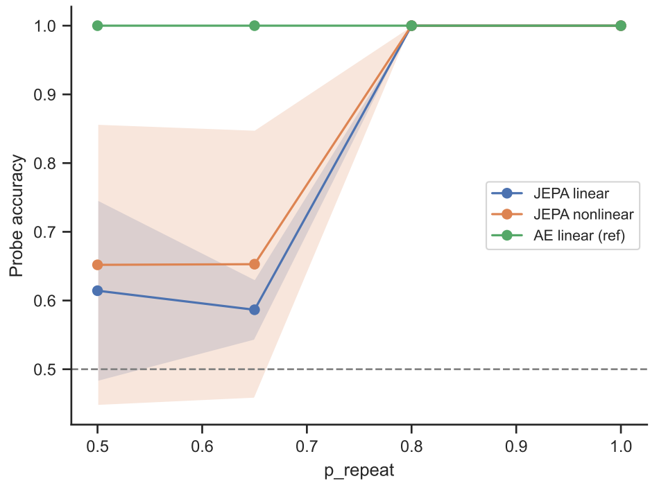
Linear vs nonlinear accessibility (JEPA)
