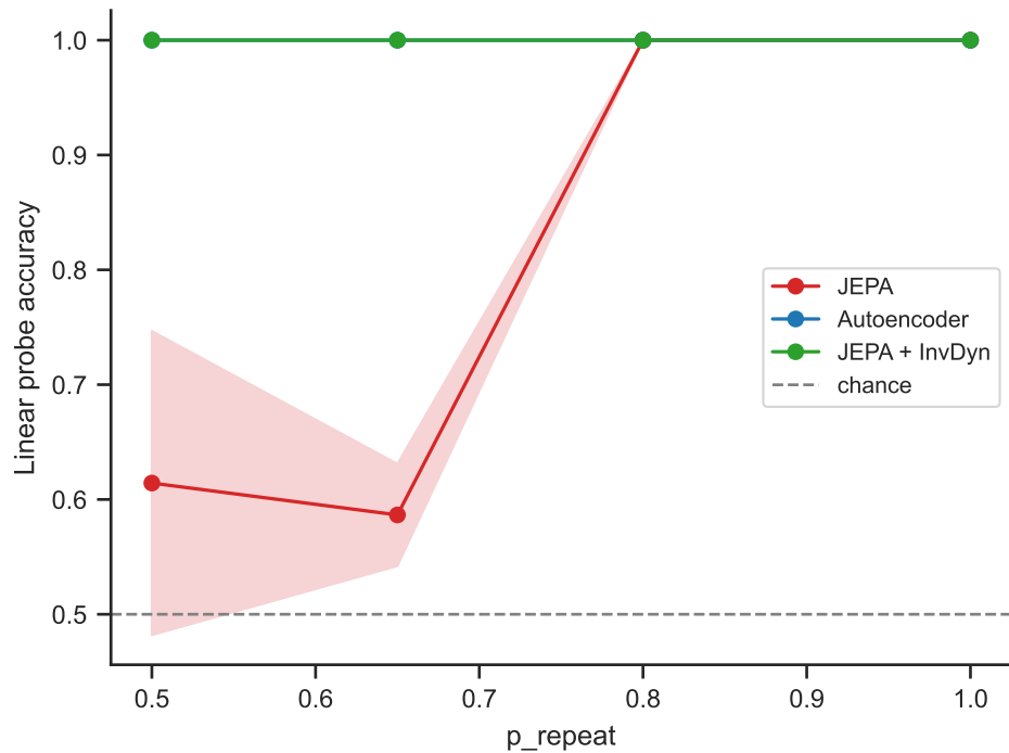
Switch color decodability vs predictability
