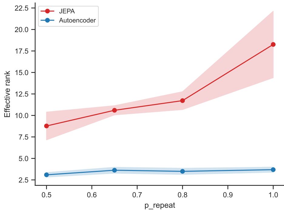
Representation rank (capacity check)
