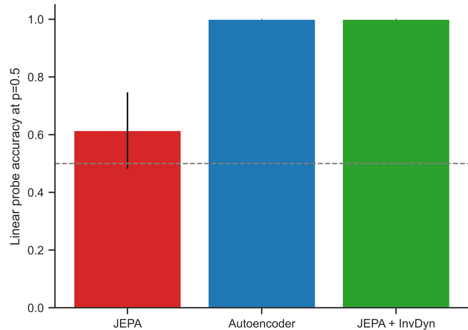
Ablation: model type at hardest setting
