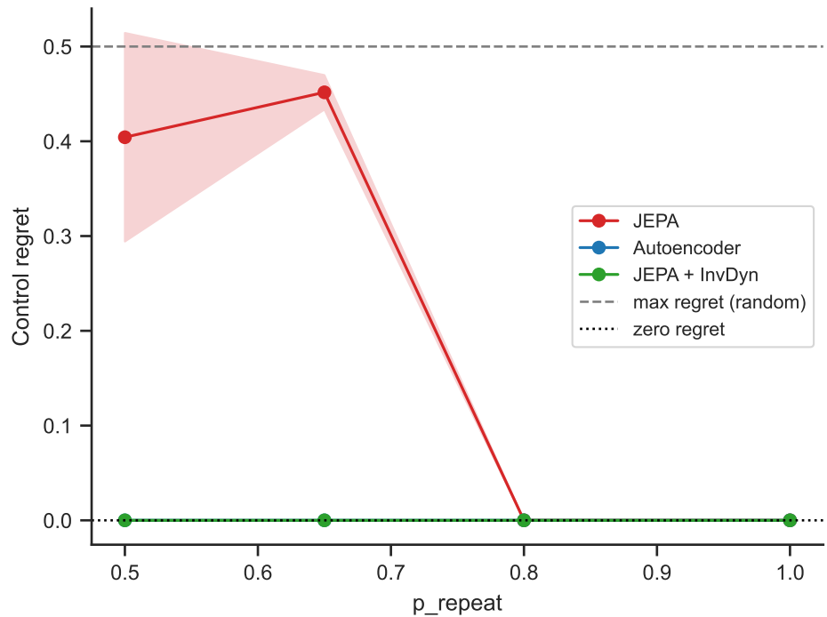
Control regret vs predictability
