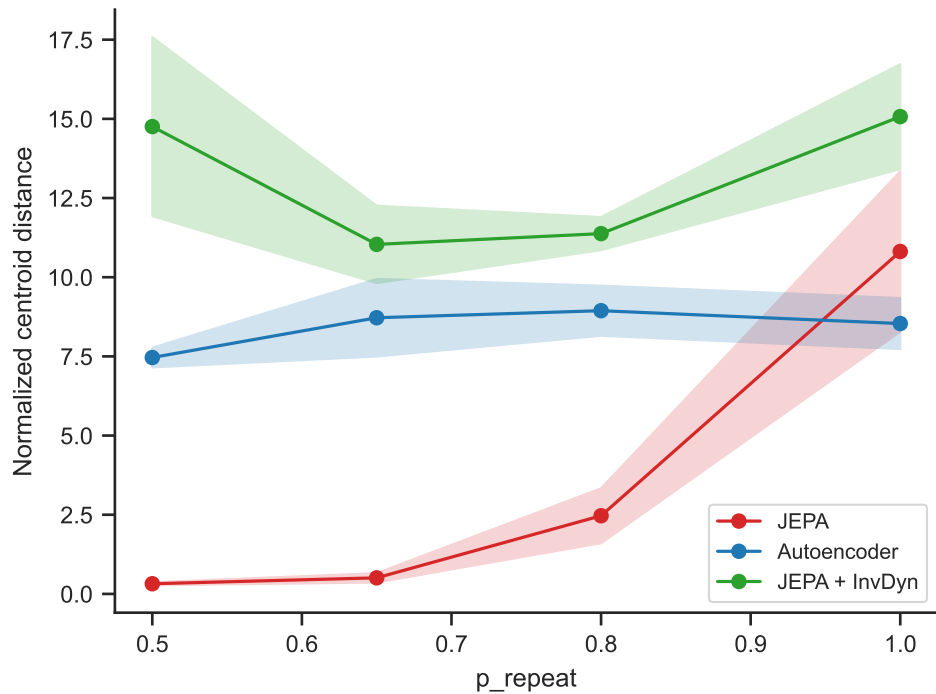
Bisimulation proxy: c=0 vs c=1 separation
