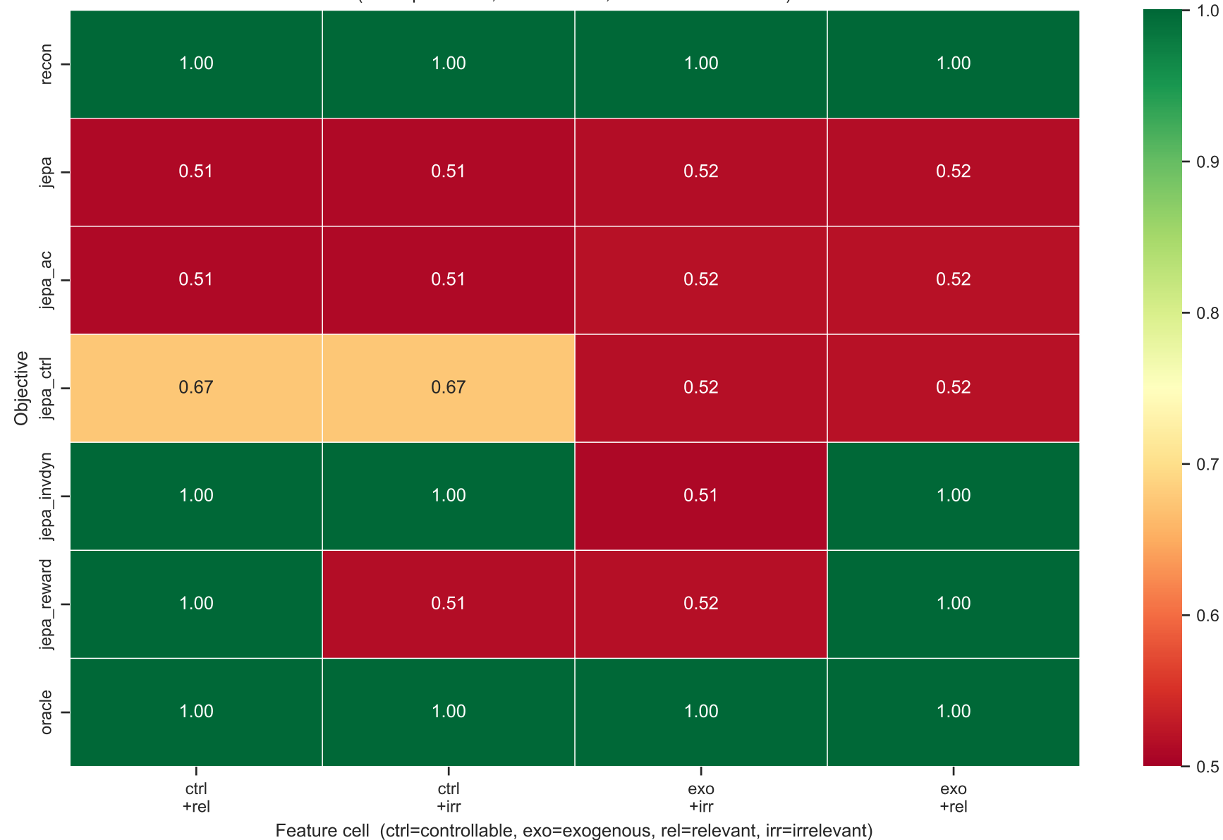
Retained feature info by objective x cell (linear probe acc, chance=0.50, retain threshold=0.75)
