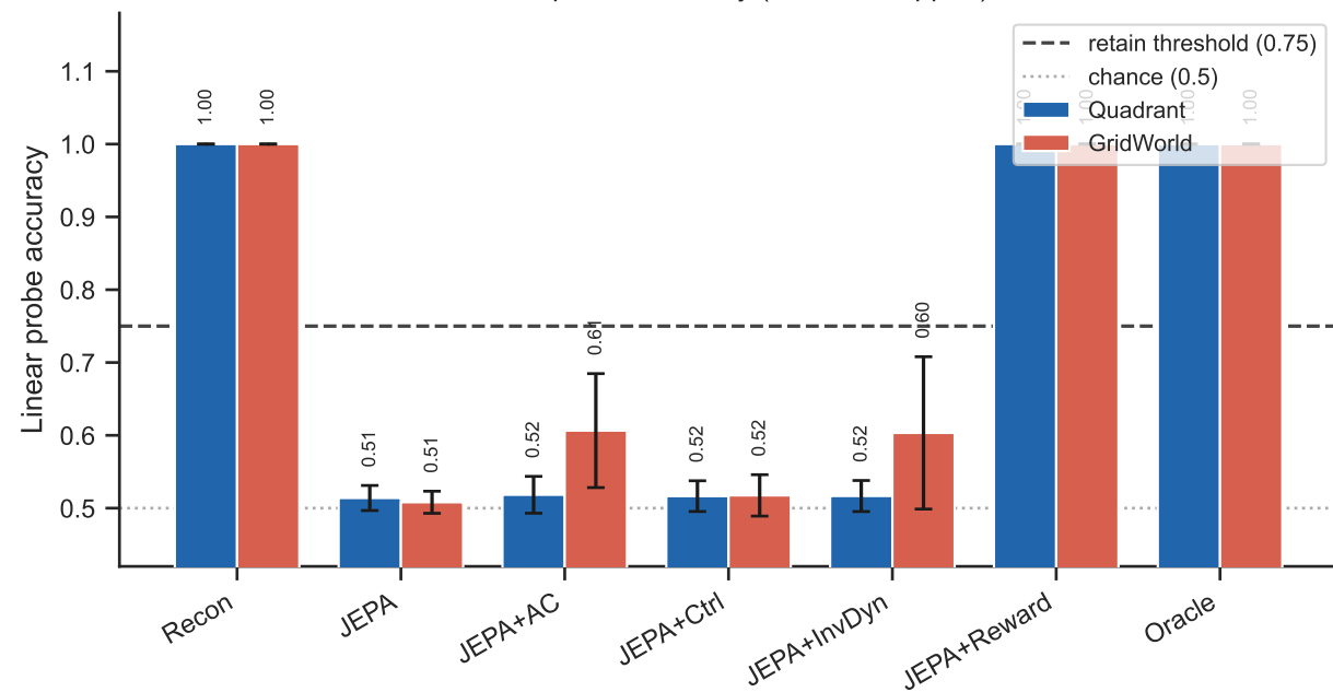
Cell-4 probe accuracy (lower = dropped)
