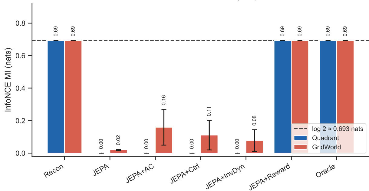
Cell-4 mutual information (nats)
