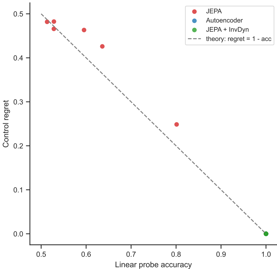
Theory vs empirical alignment
