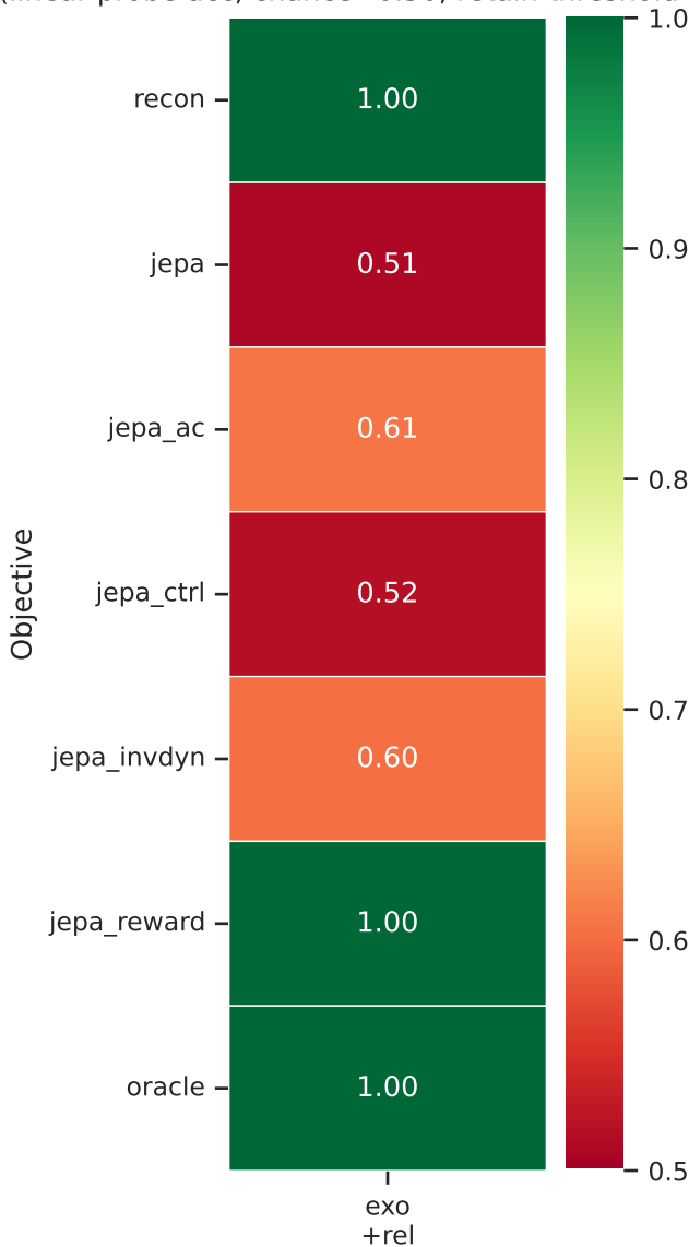
Retained feature info by objective x cell (linear probe acc, chance=0.50, retain threshold=0.75)
