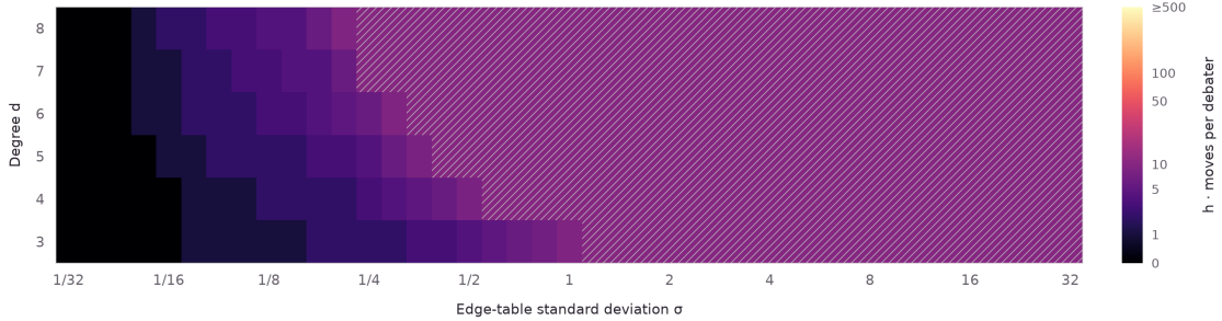
Figure 4: Integer debate budgets for target mean absolute error 0.1 on 50,000-vertex partially filled regular trees, matching the core panel. The 240 resolved cells retain simultaneous 95% confidence decisions, conditional on valid guarded numerical enclosures. Six boundary cells are assigned approximately: choose the smaller budget when its sample mean-error upper bound is at most 0.101, otherwise the larger budget. Hatching marks the cutoff h \geq 10 under this convention. The strict statistical brackets are retained separately in the figure data.
