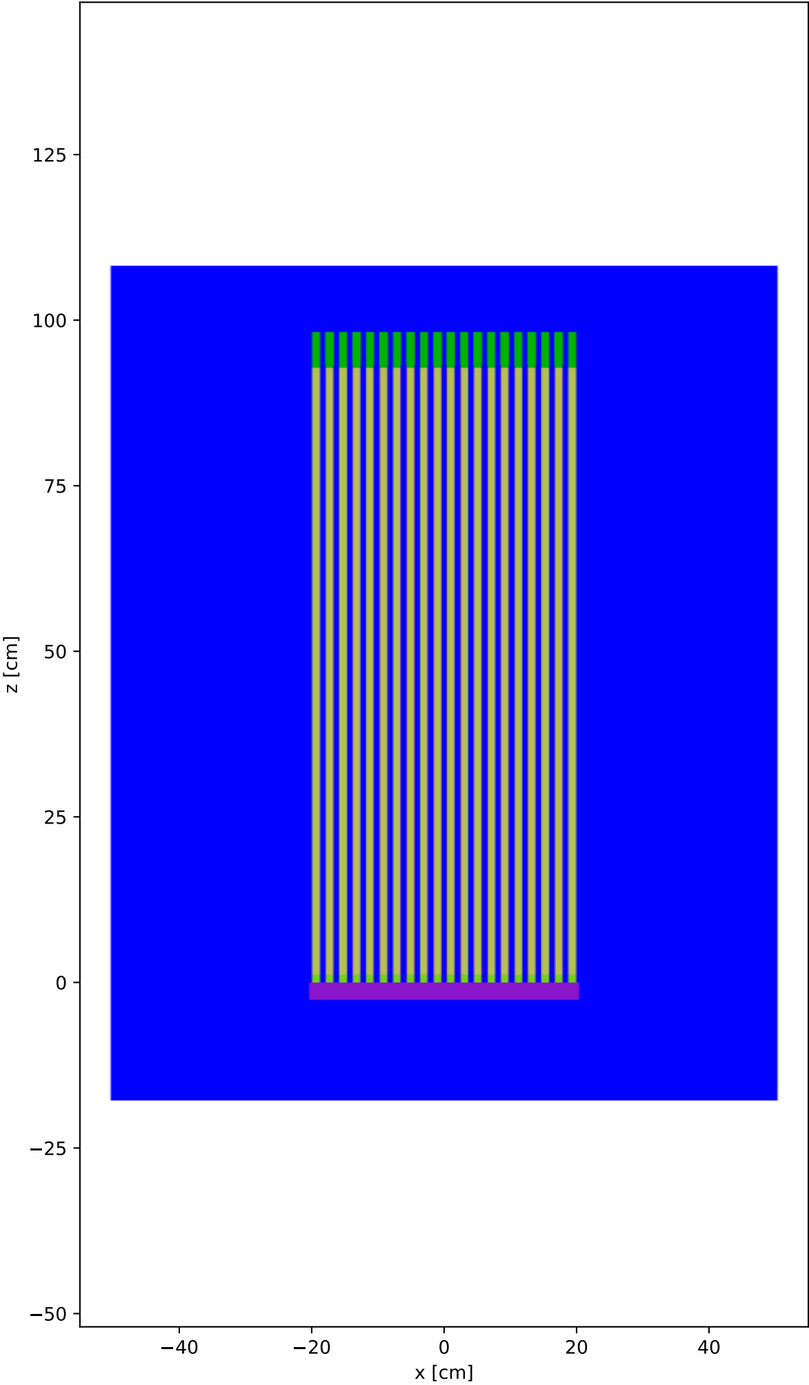
Assembly XZ View
