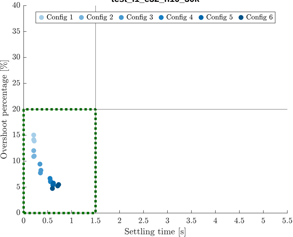
test_l1_e32_h10_30k
