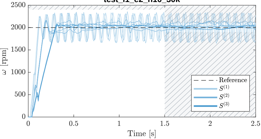
test_l1_e2_h10_30k
