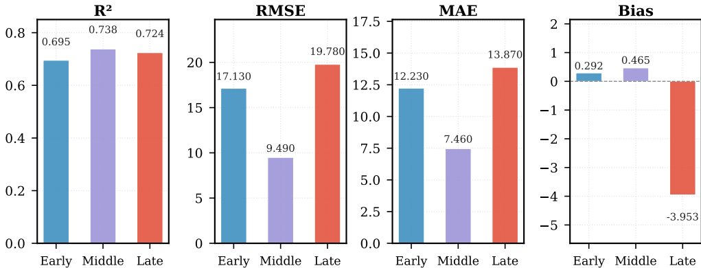
(c) LOPO CV — Period-wise Metrics
