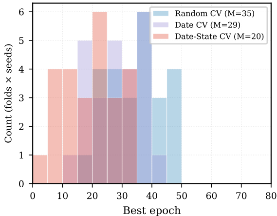
Distribution
