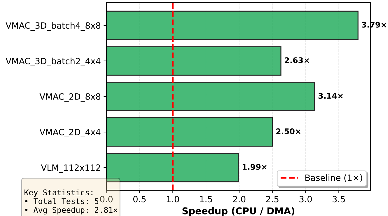
DMA Speedup over CPU Direct Write
