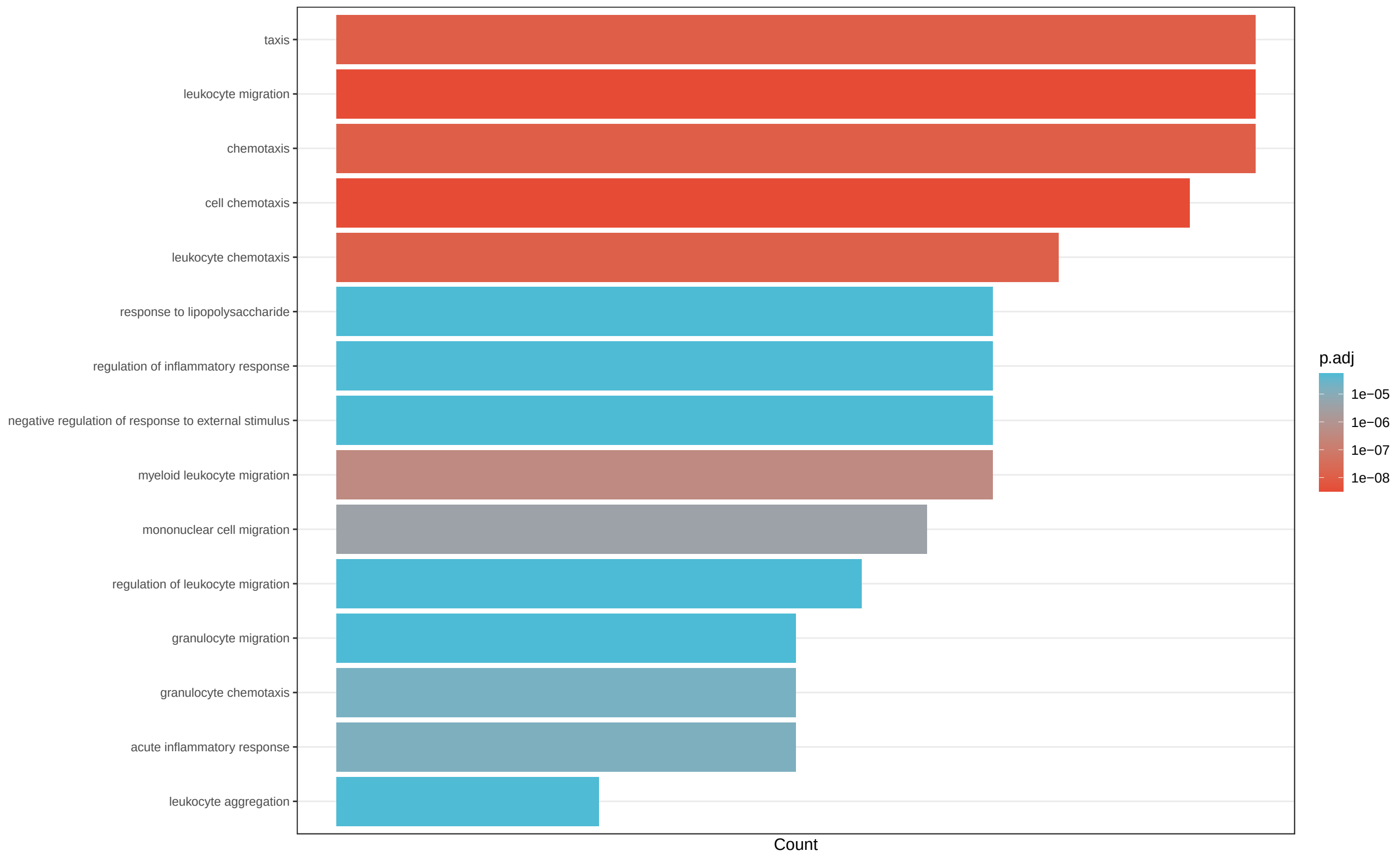
GSE190856_.... GO BP Up (bar)
