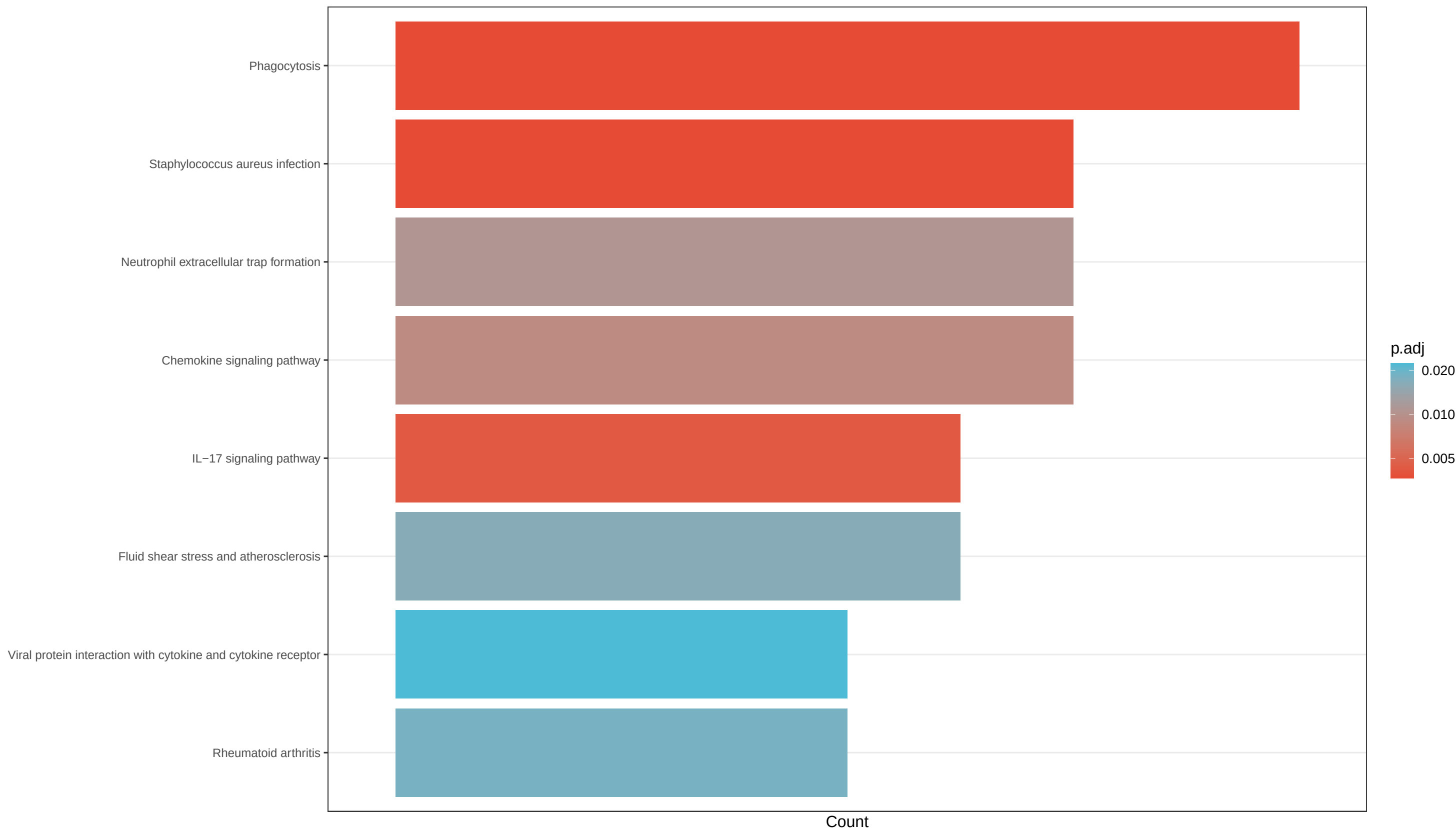
GSE190856_.... KEGG Up (bar)
