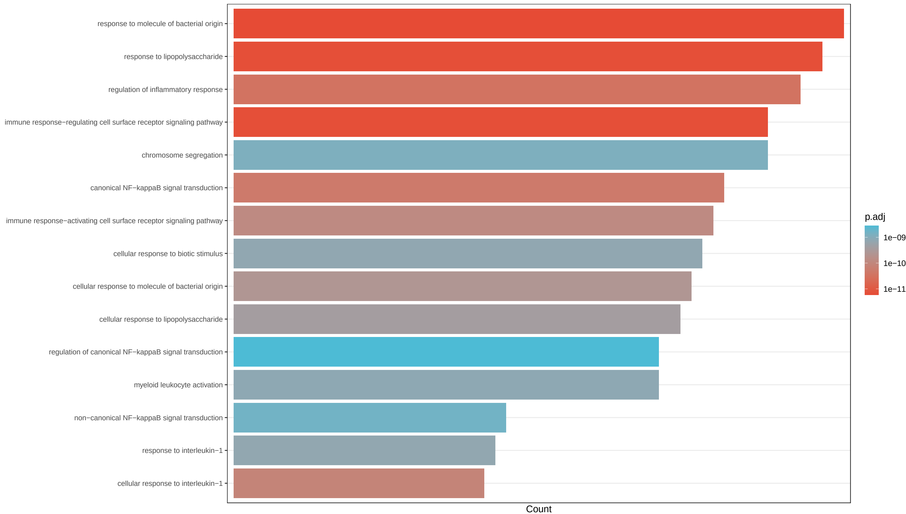
GSE207177_.... GO BP Up (bar)
