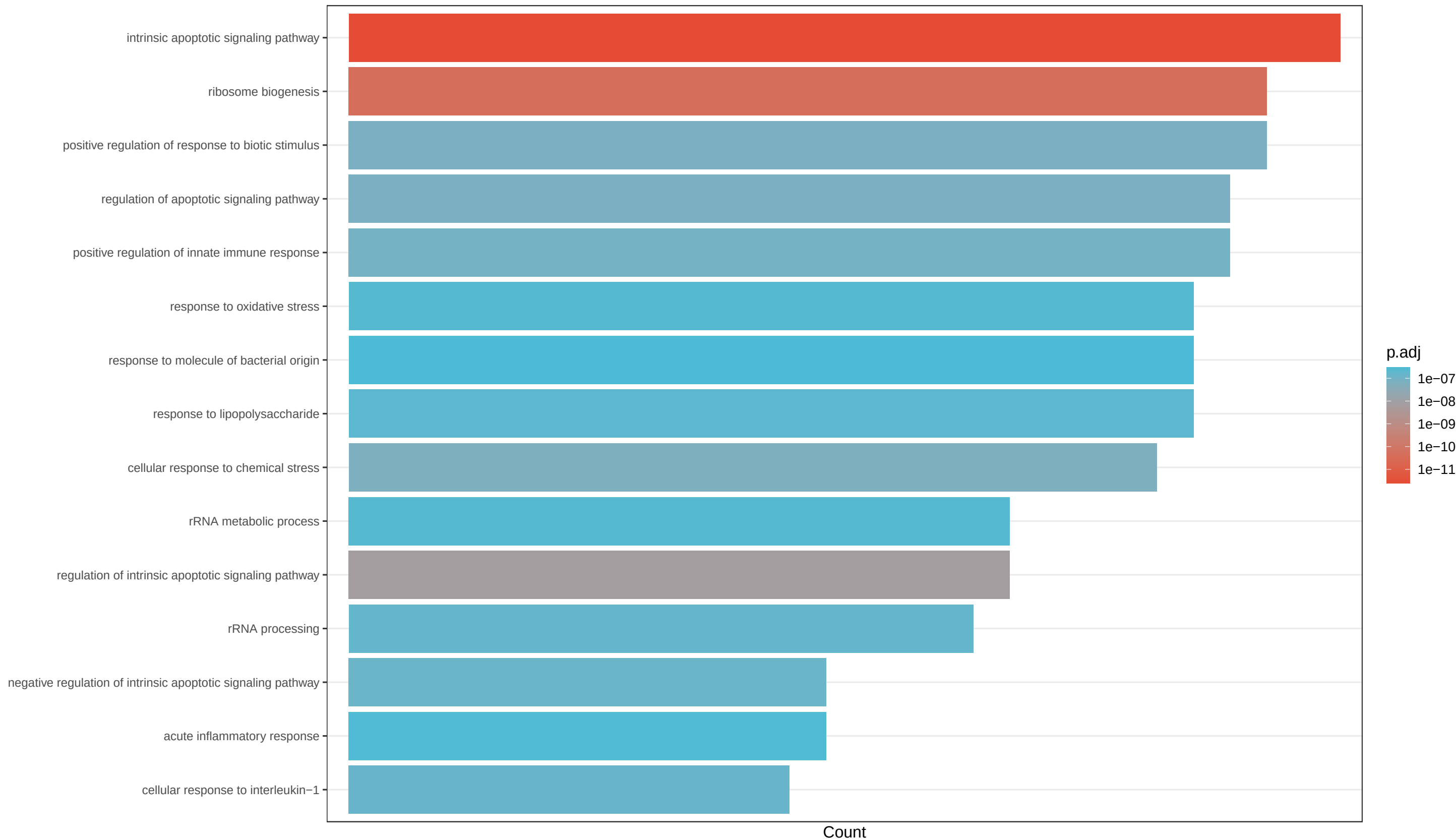
GSE207363_.... GO BP Up (bar)
