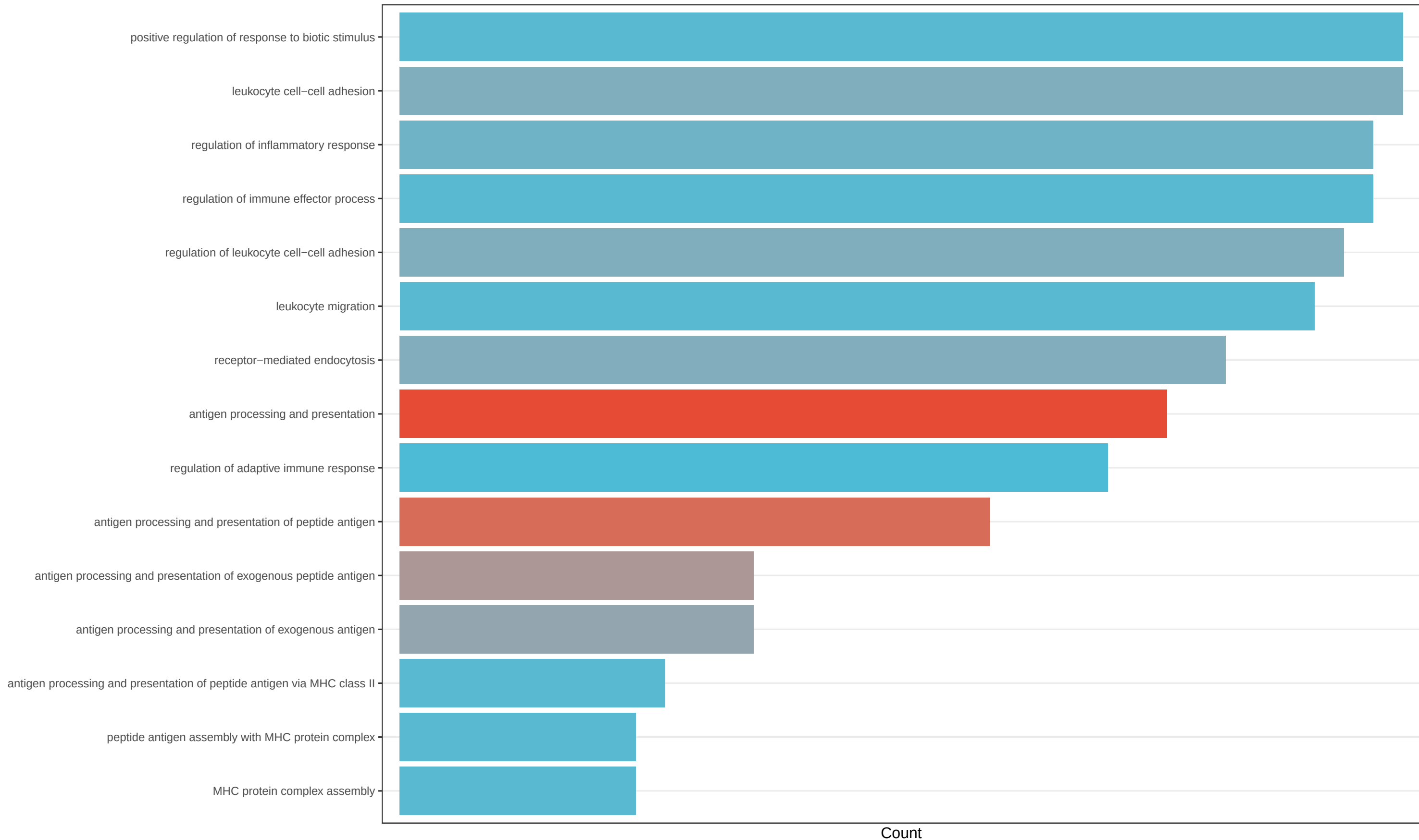
GSE207363_.... GO BP Down (bar)
