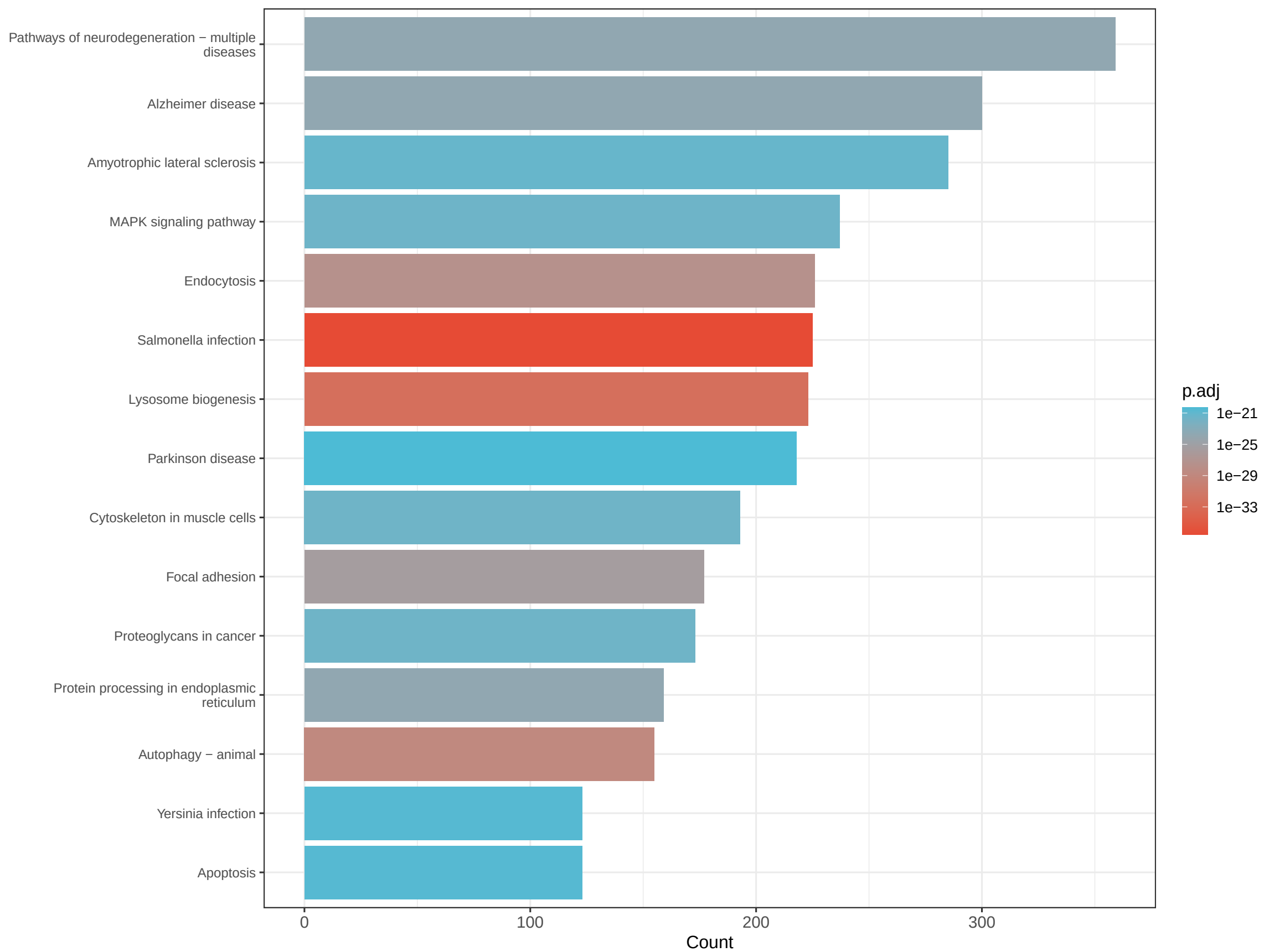
GSE267388 LPS vs PBS KEGG (bar)
