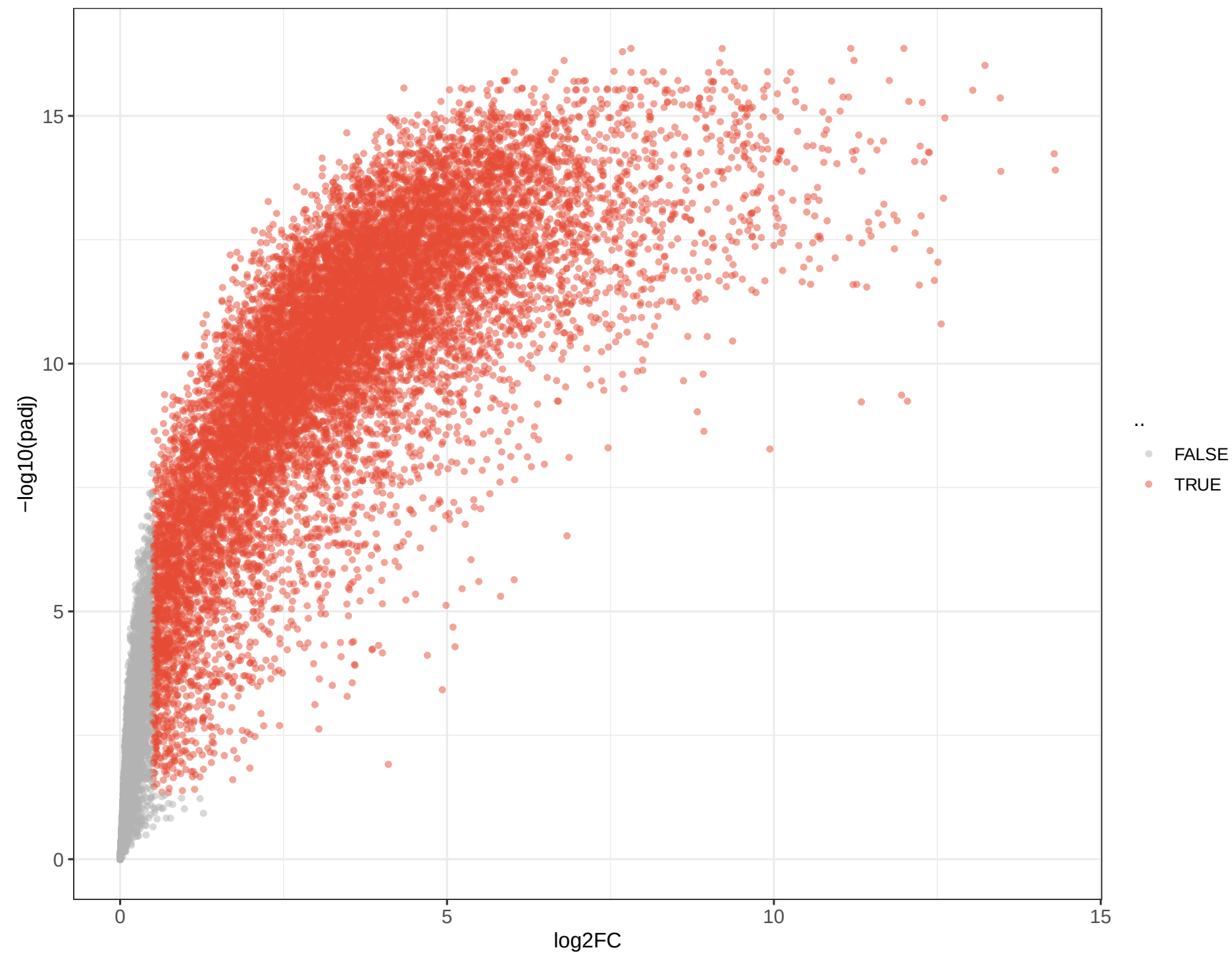
GSE267388 LPS vs PBS ...
