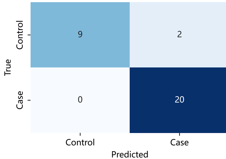
XGBoost
