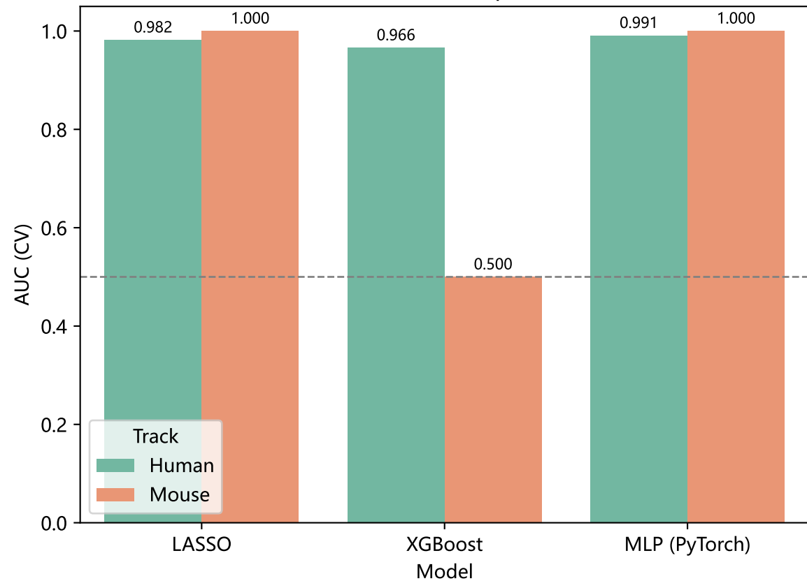
Model AUC Comparison
