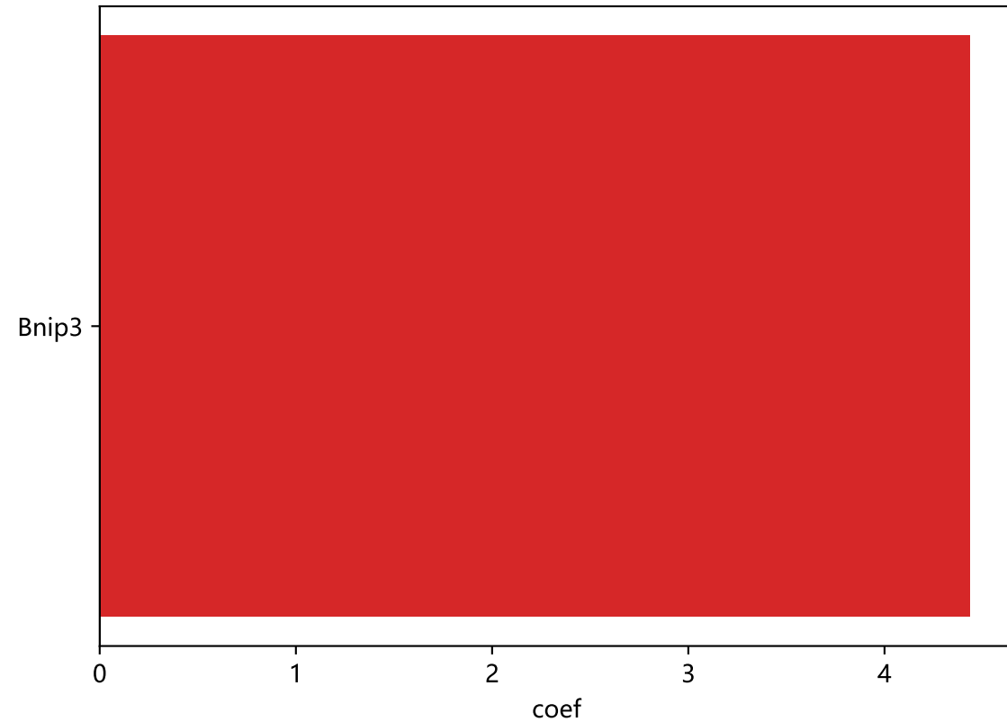
LASSO coefficients
